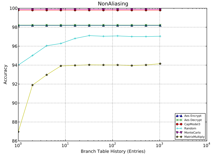
Fig. 7. Branch Predictor Accuracy
